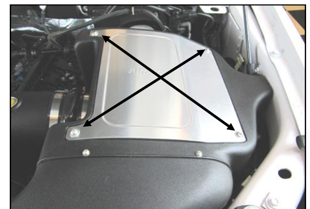
21. Mount the Lid onto the Air Box using the remaining Button Head Screws. Double check your work! Make sure all clamps, hoses, bolts, and screws are tight. Reconnect the negative battery cable!
