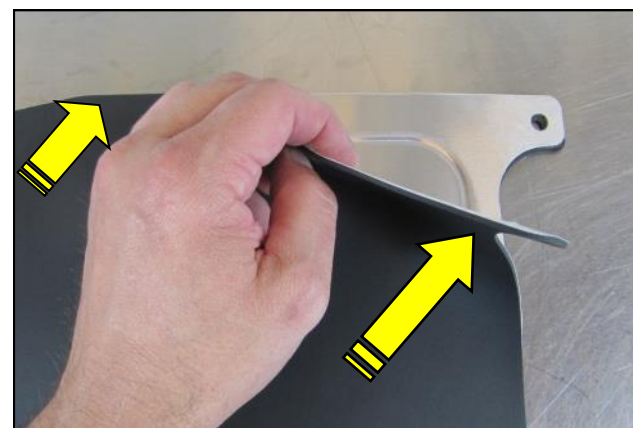
20. Remove the protective film from the top of the Air Box Lid. Prepare the underside for the Lid Gasket by cleaning it using a prep-sol or equivalent. Carefully apply the self adhesive Gasket onto the Lid as shown.
