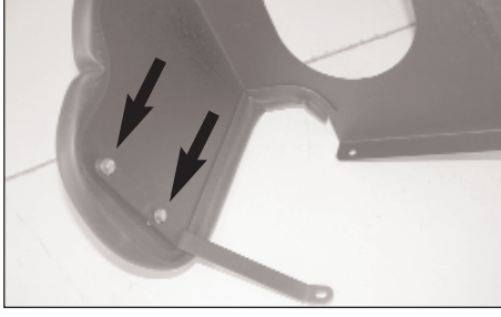
13. Using the provided hardware install the "C" bracket onto the heat shield as shown but do not tighten completely at this time.
