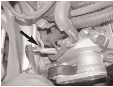
10. Remove the air conditioning hard line bolt as shown.
