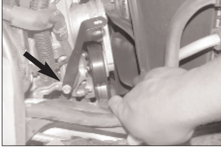
11. Using the bolt removed in step 10 secure the provided twist bracket to the original threaded boss as shown but do not tighten completely at this time.
