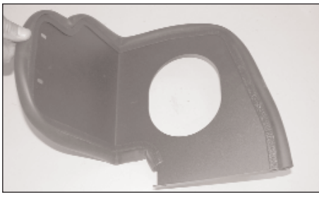
12. Install the provided trim seal onto the K&N heat shield and trim to fit as shown.
