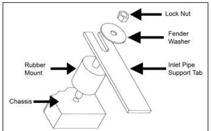
m. Proper rubber mount installation assembly.
