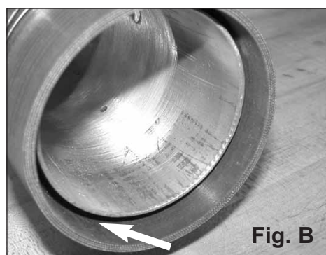
19. Please note that fig. A above denotes the correct way to install the silicone hose which has no open seal on the contact by the hose and tube. On Fig. B, this is an incorrect install of the silicone hose noting that there is an open area between the silicone hose and the intake tube.
