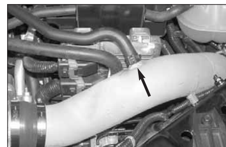
21. Reconnect the crankcase vent hose onto the K&N intake tube.
