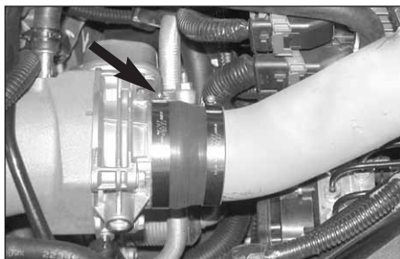
17. Install the silicone hose and provided hose clamps onto the K&N intake tube as shown.
