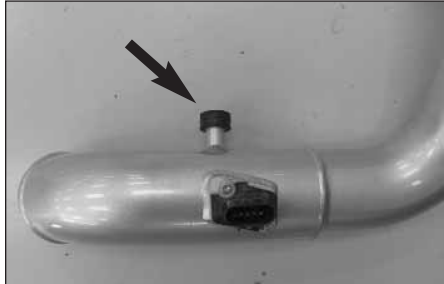
14. Install the provided rubber mounted stud onto the K&N intake tube as shown.
