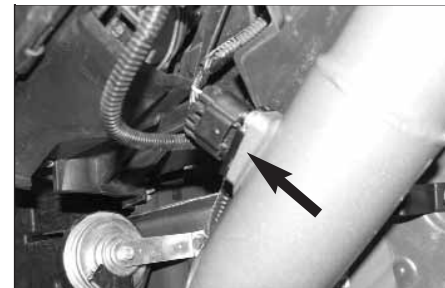
22. Reconnect the mass air sensor onto the K&N intake tube as shown.
