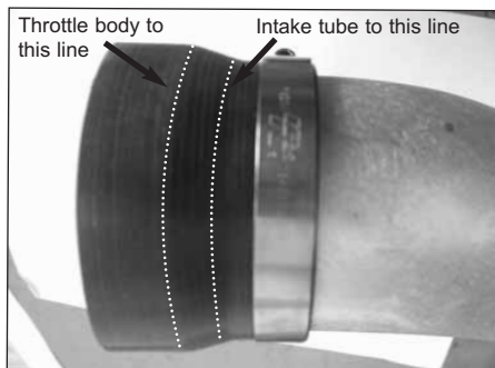
18. Slide the silicone hose and hose clamp over the throttle body then position the intake tube to where it does not go beyond the transition point of the silicone hose.
