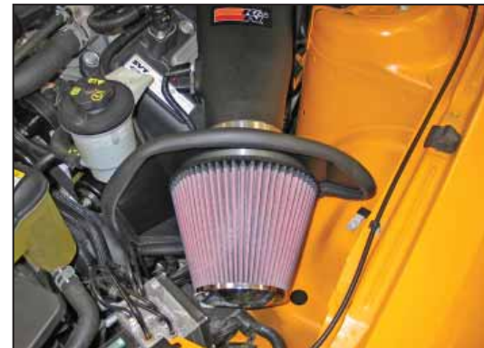
24. Set the filter assembly into the position. Slide the silicone hose onto the filter adapter's inlet and secure the filter assembly to the intake tube with the provided hose clamps.
